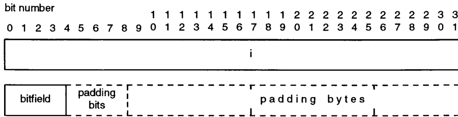
Figure 4-1. Bitfield Padding
